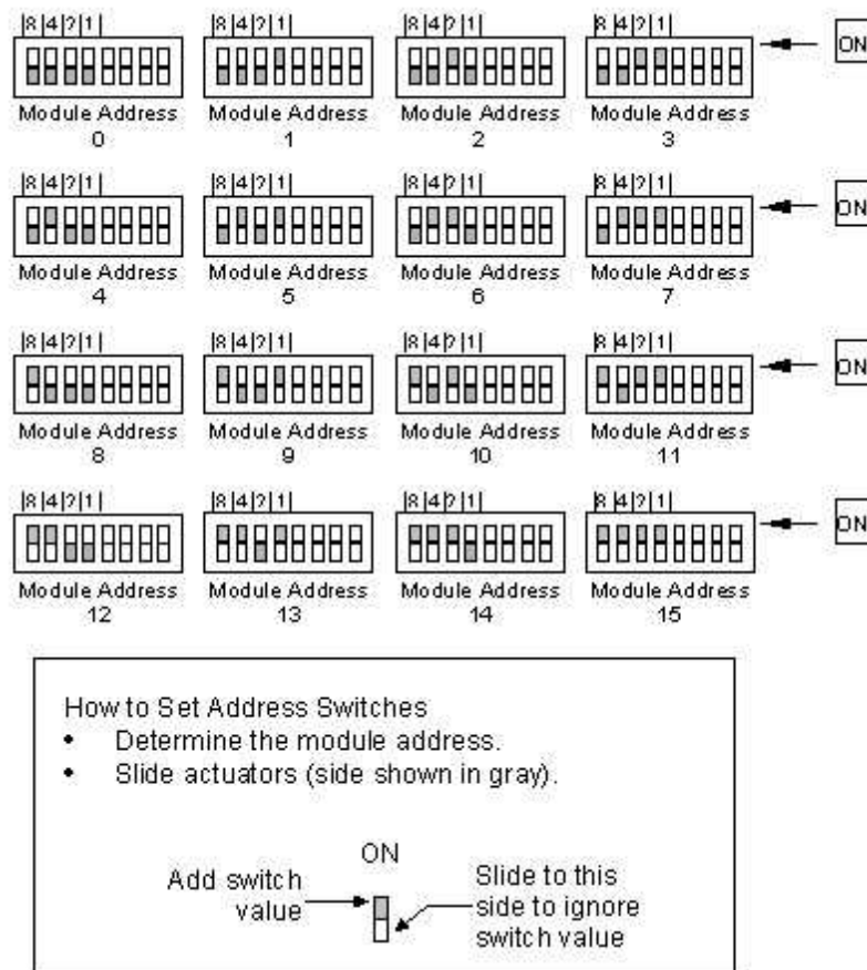
Figure 4: 5405 Digital Input Module Address Switches
