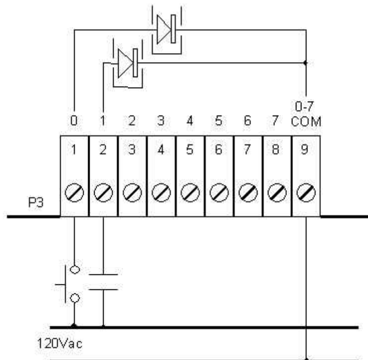
Figure 2: AC Input Wiring Example
