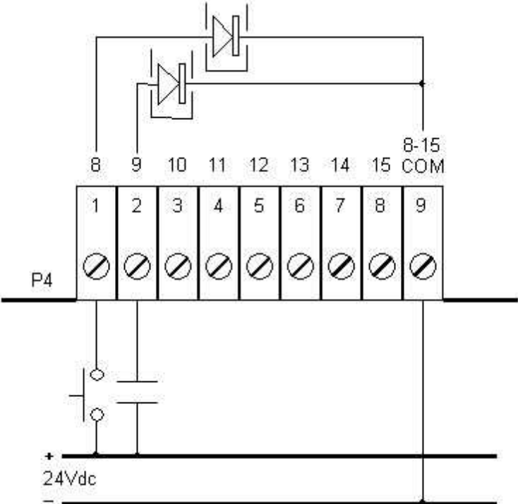
Figure 3: DC Input Wiring Example
