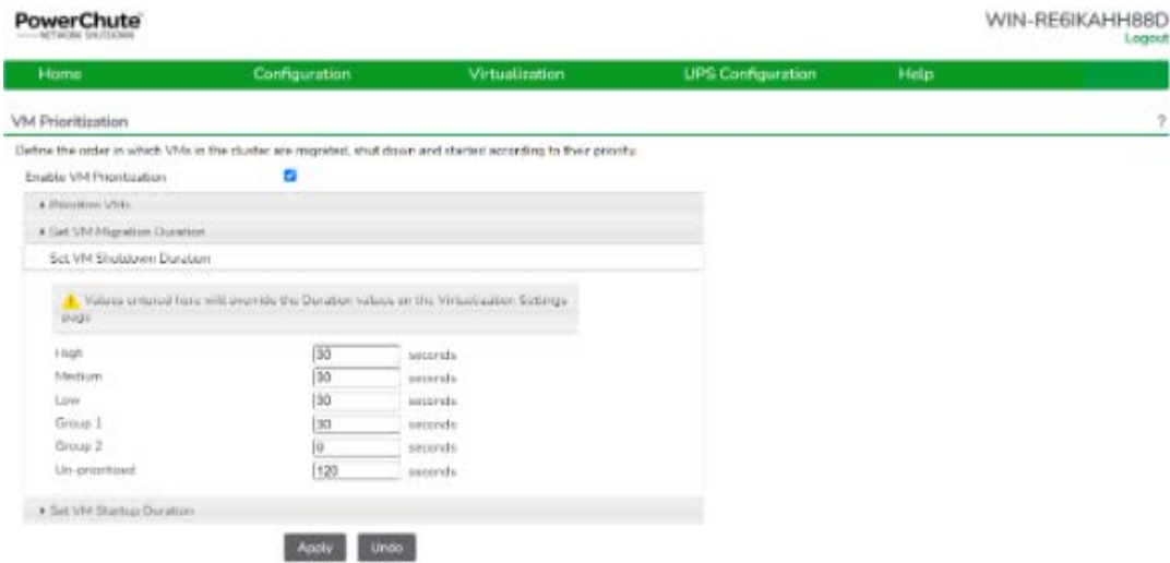
Set VM Operation durations - VM Migration, Shutdown and Startup
