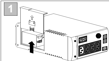
Place the unit on its side. Slide the battery compartment cover upward and off of the UPS.
