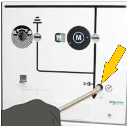
J Insert the backup handle for the switch into its hole.
