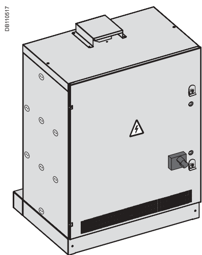
Armoire A2.
