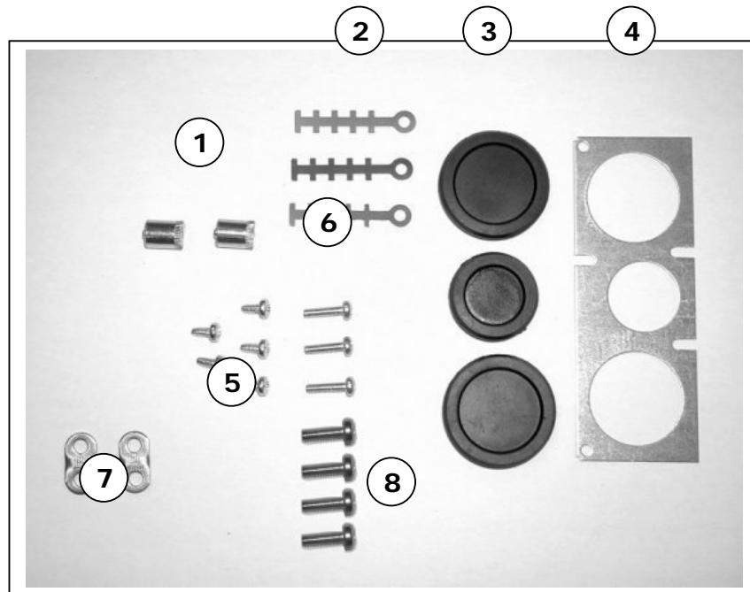
Figure 1. Cable accessories
