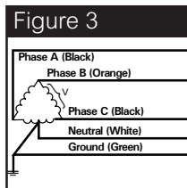
HIGH LEG DELTA (B High) 3 Phases, (B High), 1 Neutral, 1 Ground
