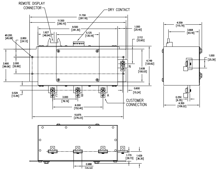
HIGH LEG DELTA (B High) 3 Phases, (B High), 1 Neutral, 1 Ground
