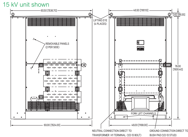
15 kV unit shown
