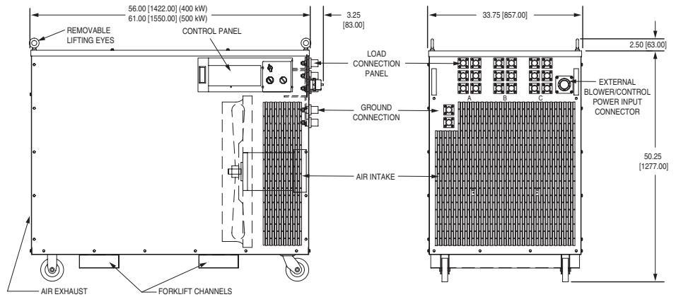
All dimensions are in inches [millimeters]. Specifications subject to change without notice.
