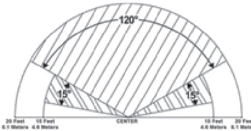
Typical horizontal detection pattern for PIR lens
