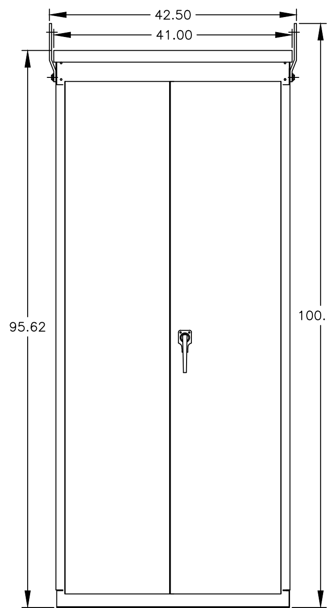
FRONT VIEW
