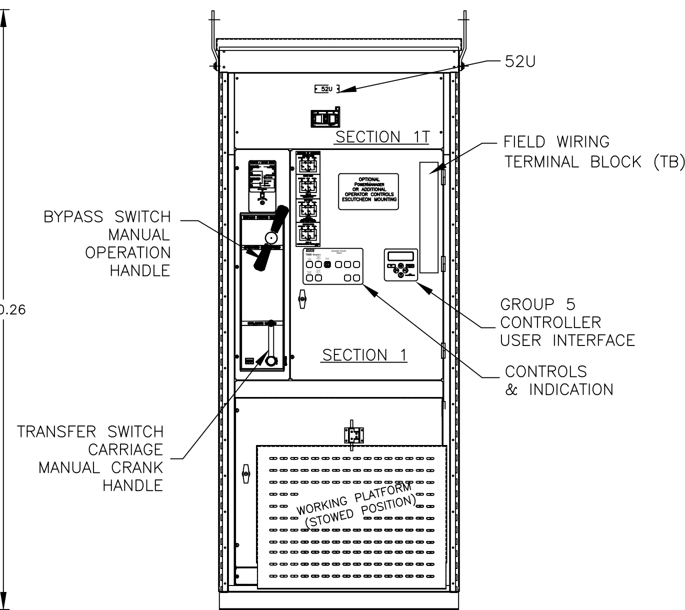
FRONT VIEW WITHOUT EXTERIOR DOORS
