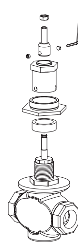
AV-802 Adapter on Johnson Controls Globe Valve
