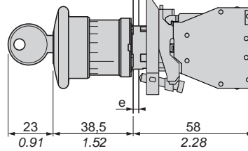
XB4BS9445GEX
