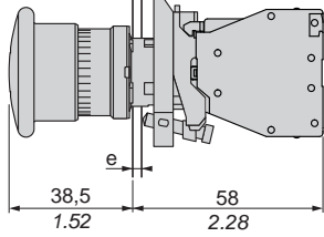
XB4BS8444GEX XB4BS8445GEX
