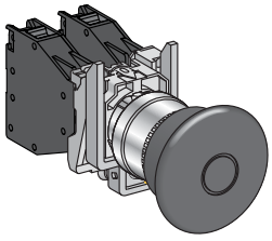
XB4BT/BS...GEX
