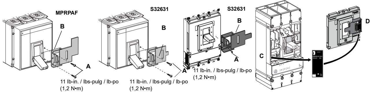
Figure / Figura / Figure 1 – Installation / Instalación / Installation
