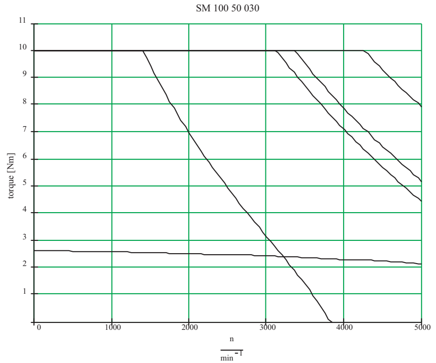
Fig. 6-11: torque-speed characteristics SM 100 50 030
