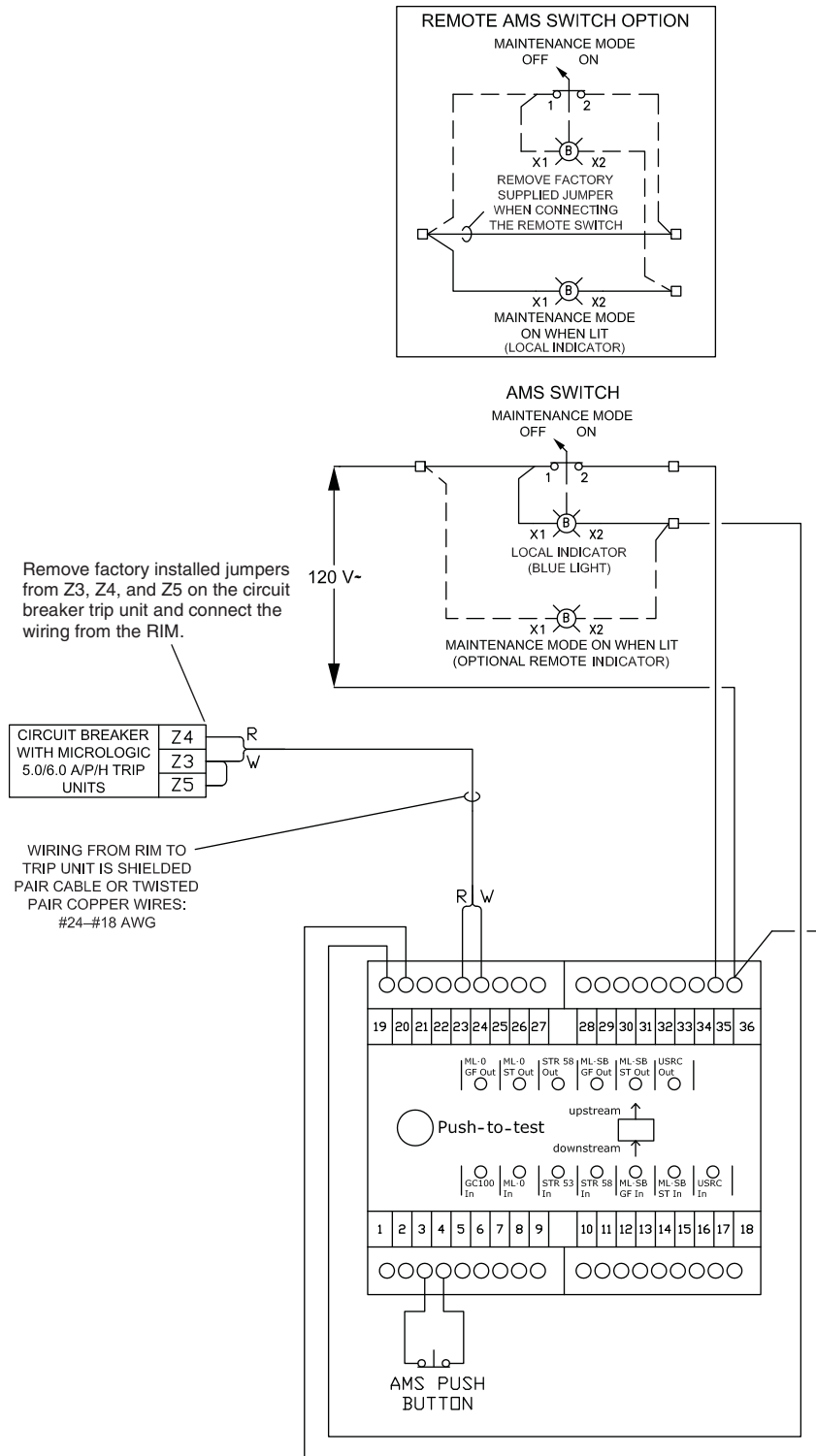
Figure 8: Wiring Diagram
