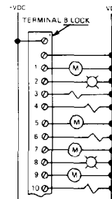
Figure 1 — Typical Wiring
