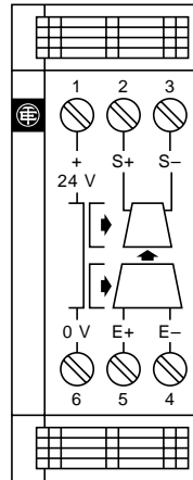
ABA-6TA●●B (isolated)
