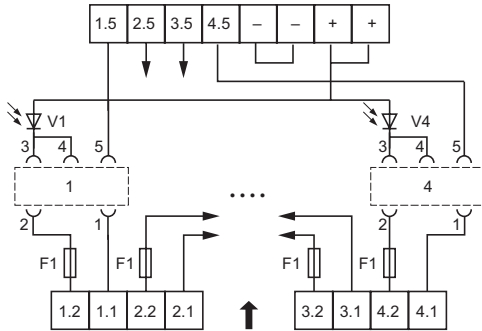
ABE-6S08E
