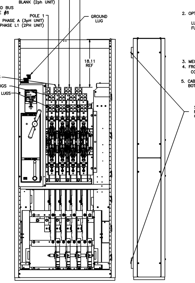
FRONT VIEW (SWITCH, DOORS, AND TOP COVER REMOVED)
