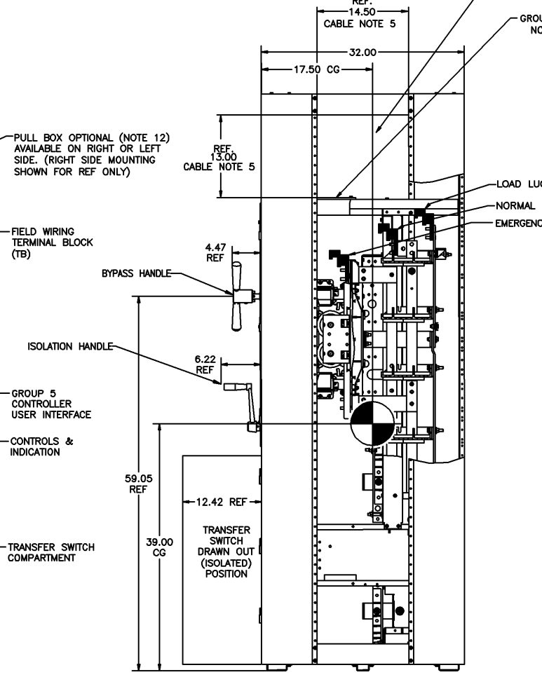
RIGHT SIDE VIEW (COVERS REMOVED AND SECTIONED FOR CLARITY)
