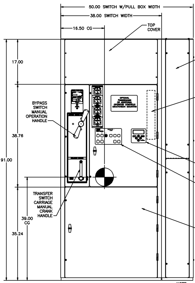
FRONT VIEW (DOORS AND TOP COVER INSTALLED)
