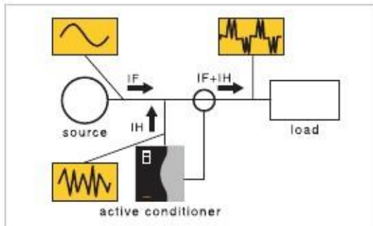
SineWave/AccuSine
