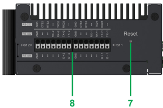
Top view of Harmony BX1
