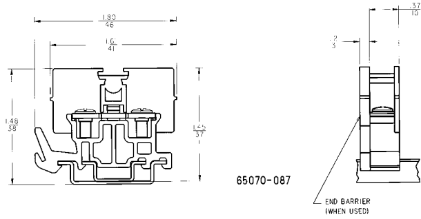
Type GA6
