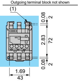
Panel mounting Outgoing terminal block not shown
