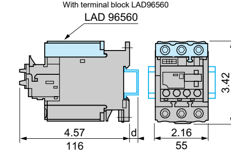
LRD313-365 Mounting on rail AM1D•200 or ED200 With terminal block LAD96560
