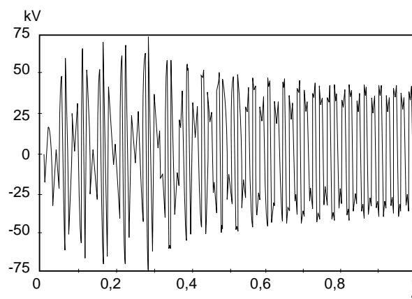
b - VT primary voltage in kilovolts (kV) over time in seconds (s). The voltage shows a complex, oscillatory waveform with significant amplitude, characteristic of ferroresonance. The y-axis ranges from -75 to 75 kV, and the x-axis ranges from 0 to 1.0 s.
