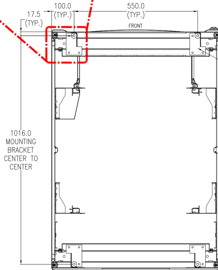
BOTTOM VIEW (AR3140) WITH CHANNEL MOUNTING BRACKET KIT (AR7709)
