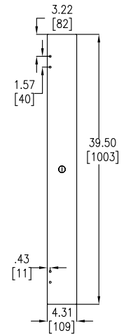
PART "I" - FRONT VIEW
