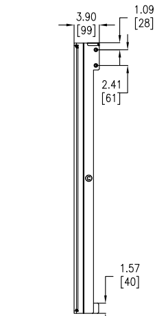
PART "C" - SIDE VIEW
