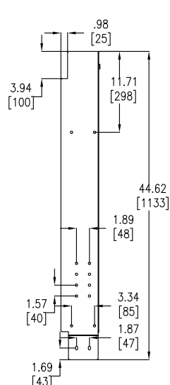
PART "K" - FRONT VIEW
