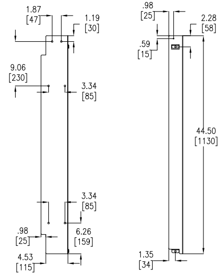
PART "J" - FRONT VIEW
