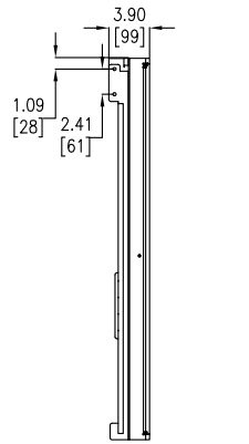
PART "A" - SIDE VIEW
