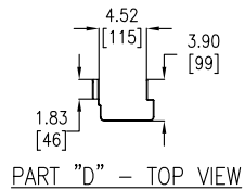
PART "D" - TOP VIEW
