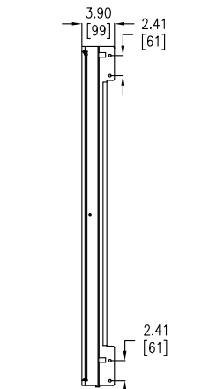
PART "B" - SIDE VIEW
