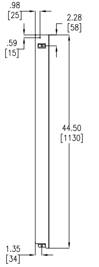
PART "J" - SIDE VIEW
