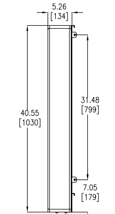
PART "B" - FRONT VIEW
