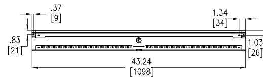
PART "E" - FRONT VIEW
