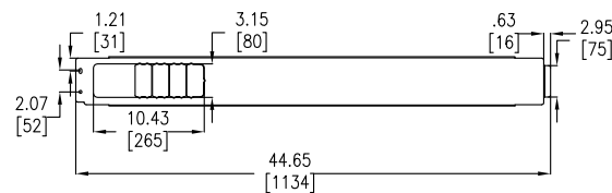
PART "F" - FRONT VIEW
