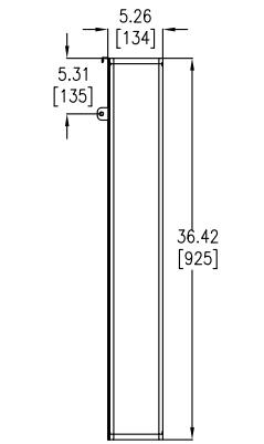
PART "A" - FRONT VIEW
