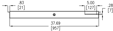
PART "G" - SIDE VIEW
