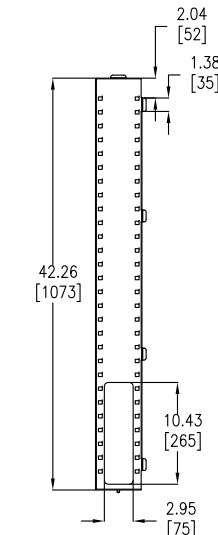
PART "L" - TOP VIEW
