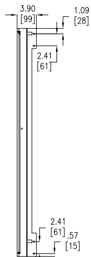
PART "D" - SIDE VIEW
