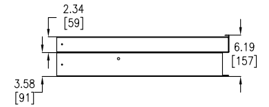
PART "N" (ASSEMBLED) - SIDE VIEW
