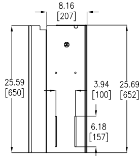
PART "N" (ASSEMBLED) - TOP VIEW
