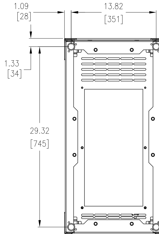
LEVELER LOCATIONS BASE TOP VIEW
