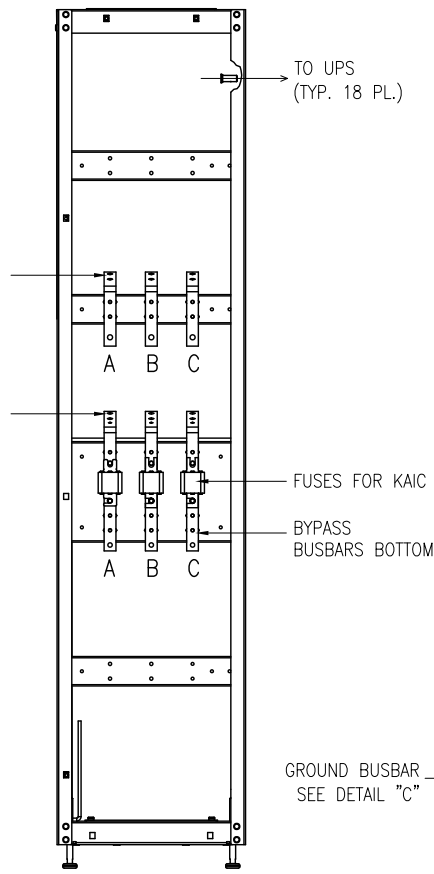
FRONT VIEW BOTTOM ENTRY
