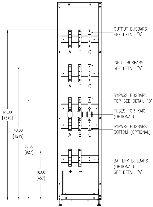
FRONT VIEW TOP ENTRY
