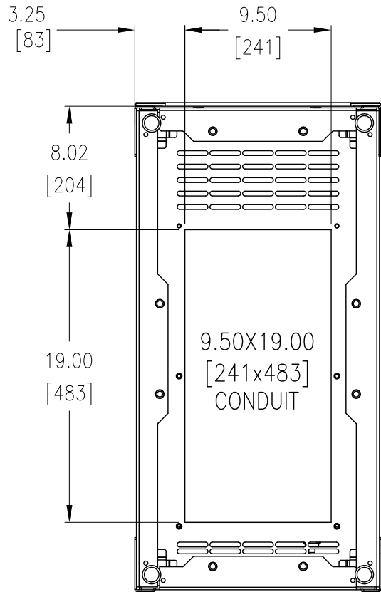
BOTTOM ENTRY CONDUIT LOCATION BASE TOP VIEW
