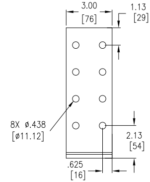
DETAIL "C" GROUND BUSBAR
