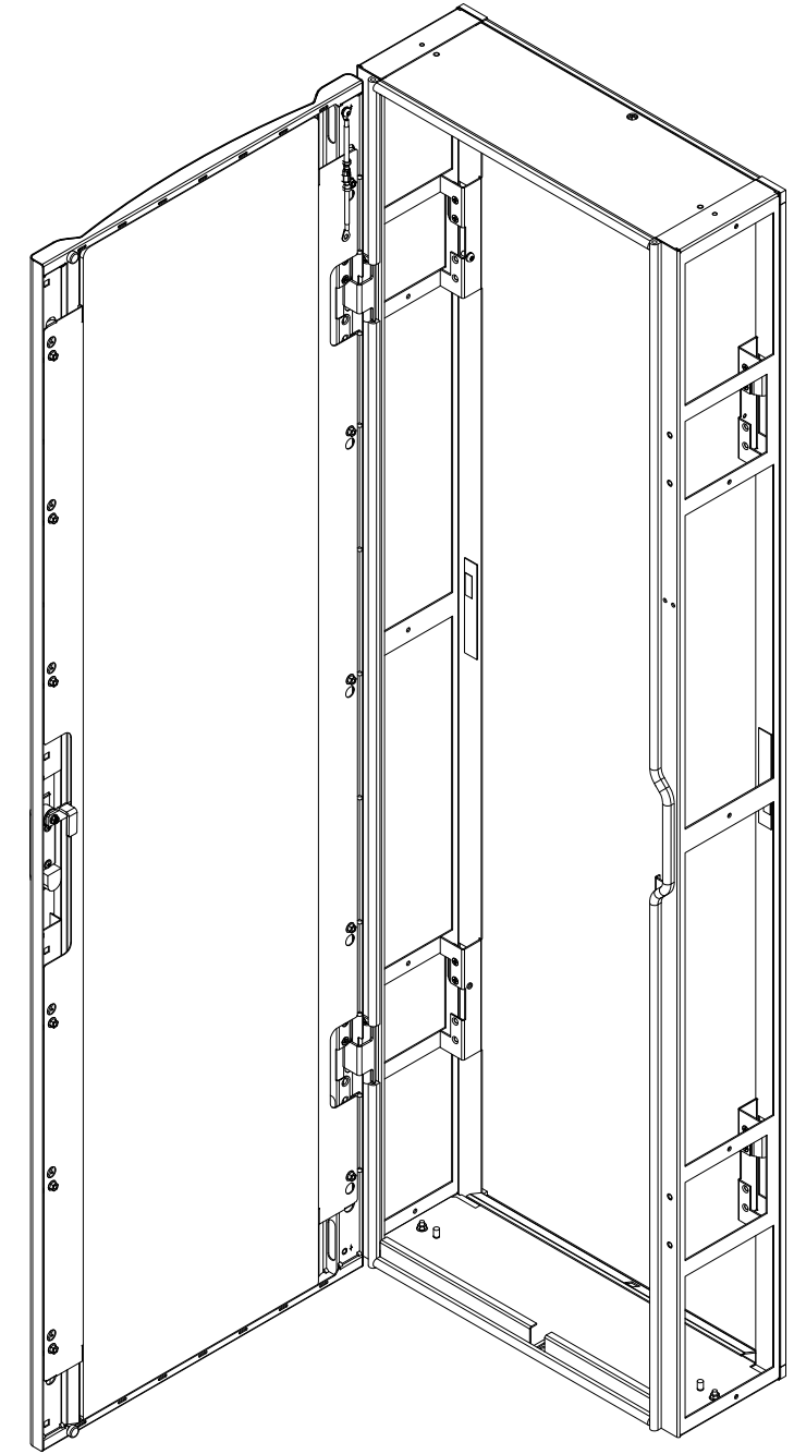
ISOMETRIC VIEW DOOR OPEN
