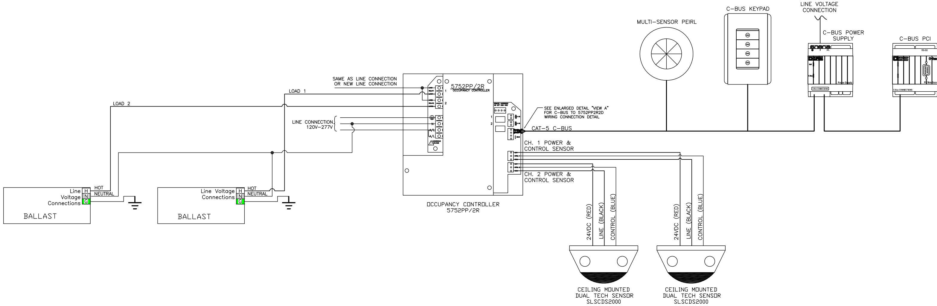
VIEW A
