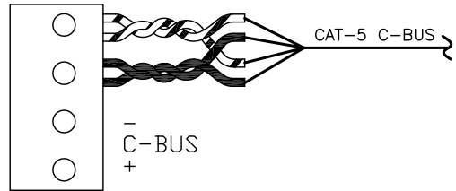
VIEW A
