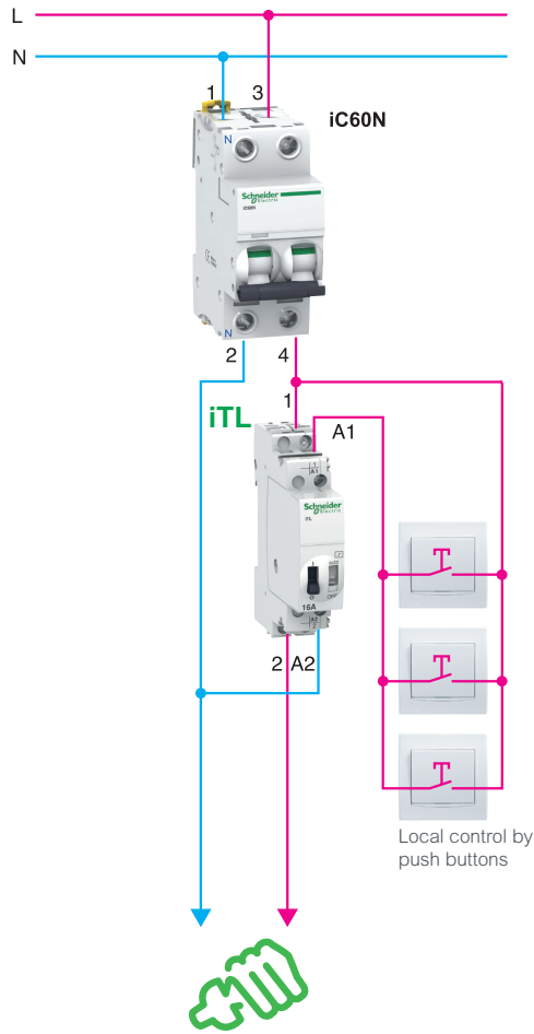
Lighting for a meeting room
