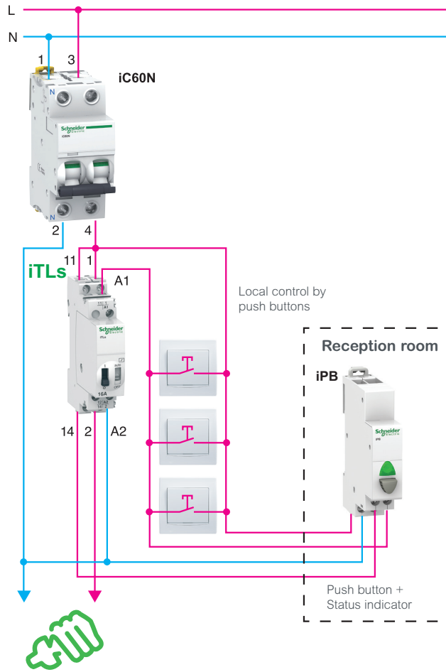
Lighting for a meeting room Variant with remote reporting (circuit status)
