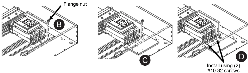
Mounting pan extension and #10-32 screws
