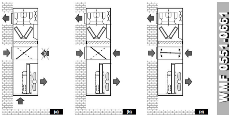
Mechanical Cooling
