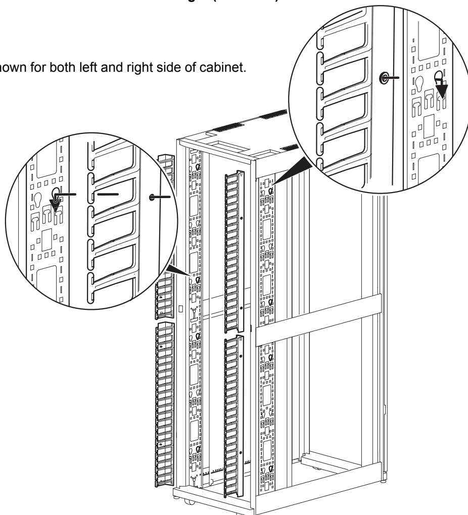
Vertical Cable Manager (1 of each)
