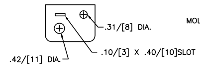
SEAL BRACKET
