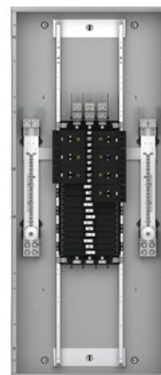
NF 600A 3P4W MLO Panelboard with Condo Riser Neutral Assembly
