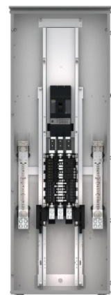
NQ 600A 3P4W MB Panelboard with Condo Riser Neutral Assembly
