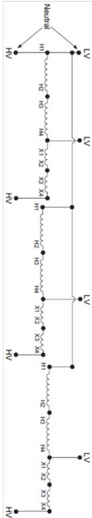
Wiring Diagram 10
