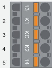
SIM-Klemmenblock
