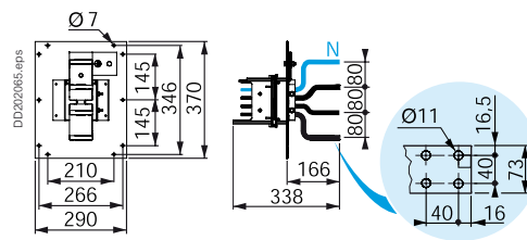
KSA1000AE4
