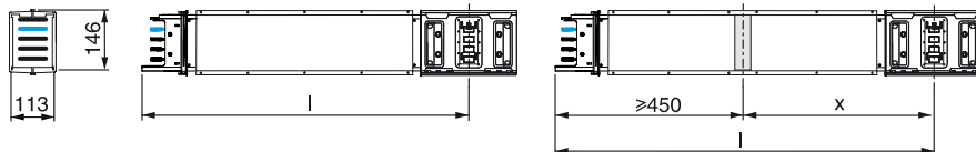
KSA1000ET4A
