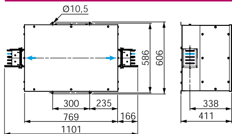
KSA1000ABT4
