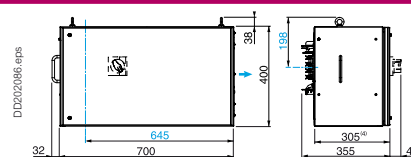
KSB400DC●TRE
