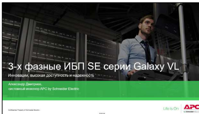
Galaxy VL
