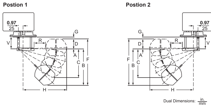
Figure 23: Travel Dimensions
