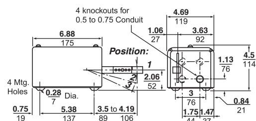
Figure 18: Type AG1 Dimensions
