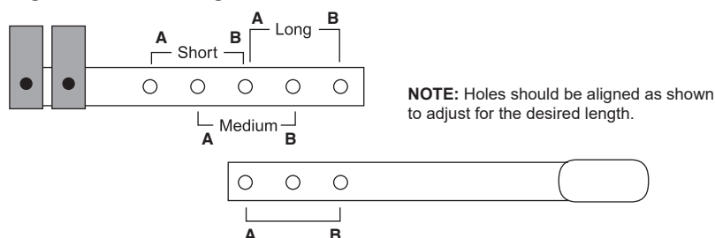
Figure 3: Lever Length
