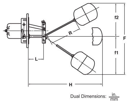
Figure 12: Float Position 3
