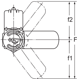
Figure 13: Travel Dimensions
