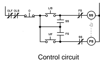
Control circuit
