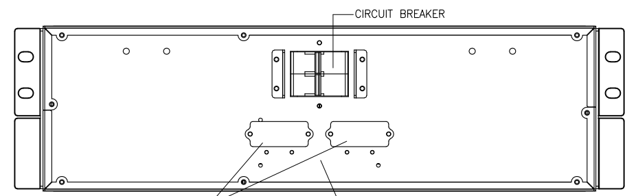
BATTERY CONNECTOR (COVER NOT SHOWN) GROUND SCREW
