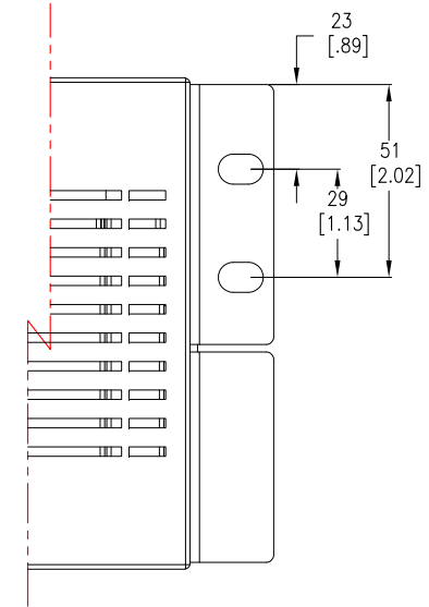
DETAIL-A (ENLARGED)
