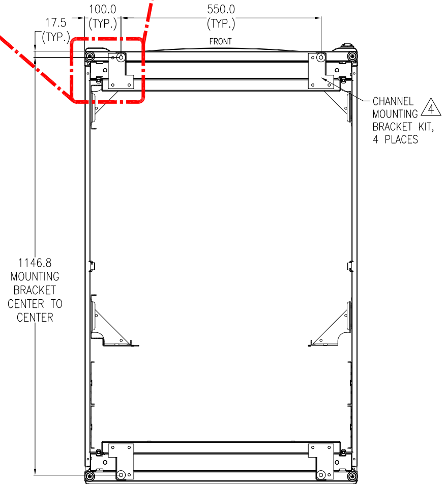
BOTTOM VIEW (AR3355)
