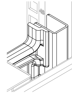
ENLARGED RIGHT-SIDE MOUNTING DETAIL-C
