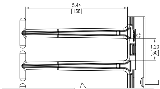
TYPICAL ENLARGED RIGHT SIDE VIEW DETAIL-A
