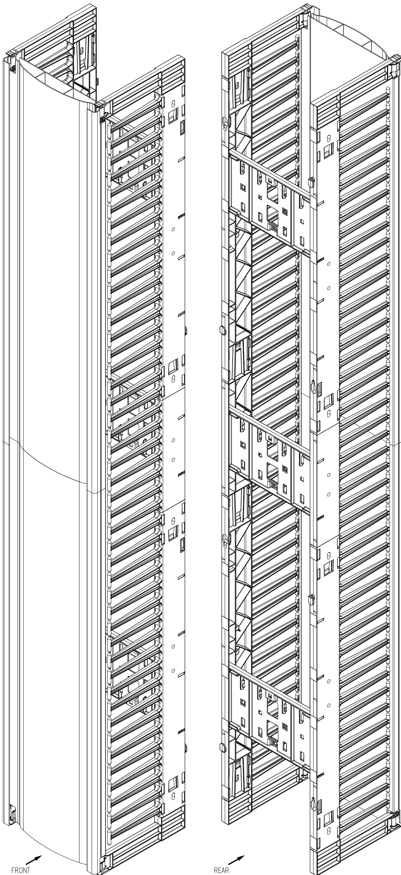
ISOMETRIC VIEW
