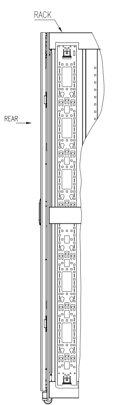
TYPICAL MOUNTING INSIDE THE RACK (RACK SIDE COVERS REMOVED)
