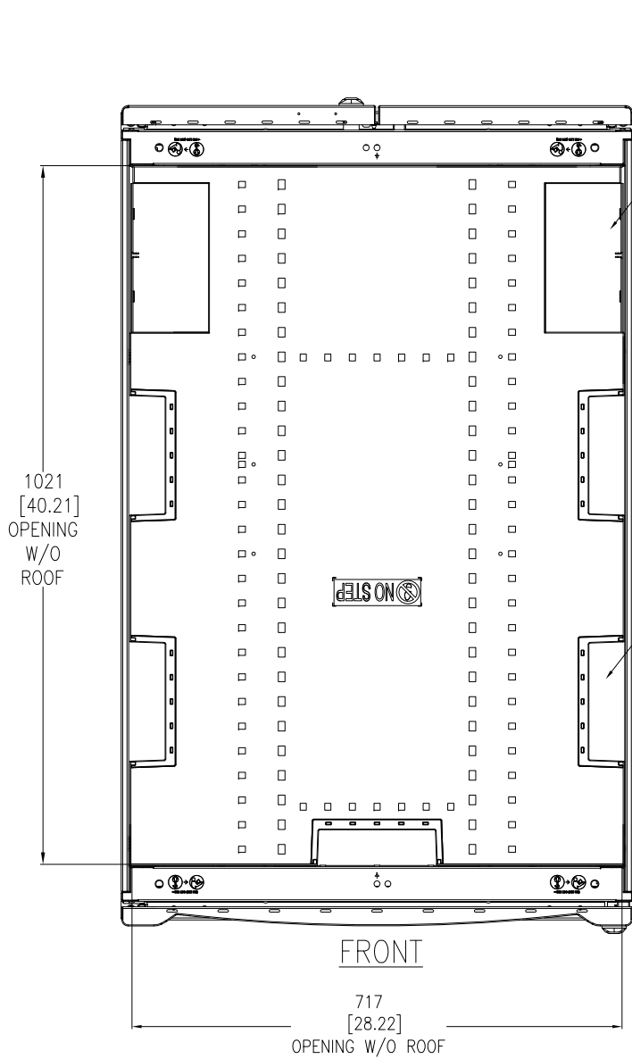
TOP VIEW CABLE OPENINGS (COVERS REMOVED)
