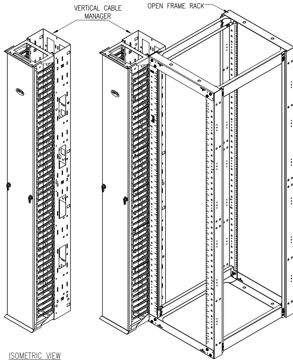
TYPICAL APPLICATION (ISOMETRIC VIEW)
