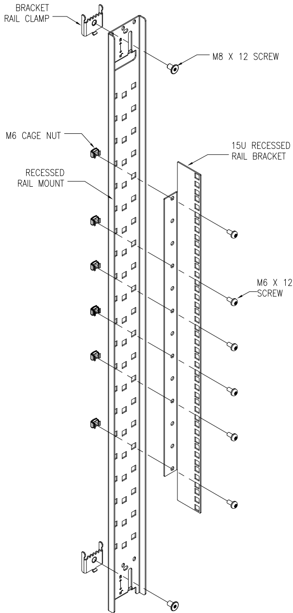
ISOMETRIC VIEW WITH 15U RECESSED RAIL BRACKET (EXPLODED VIEW)
