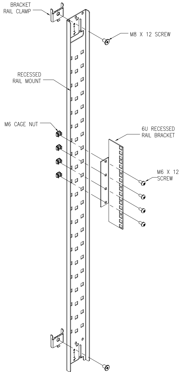
ISOMETRIC VIEW WITH 6U RECESSED RAIL BRACKET (EXPLODED VIEW)
